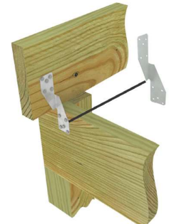
Typical RT7A installation
